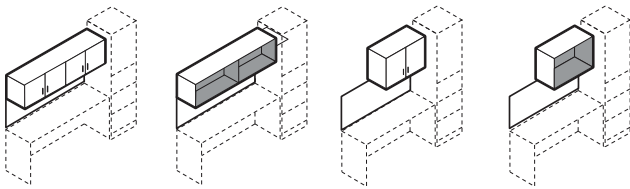
ZWHTxx25 ZxxS160S/OSN - 71.5"/72" overall
